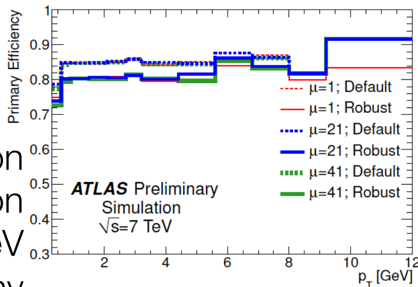
(a) Primary track reconstruction efficiency vs p_T
