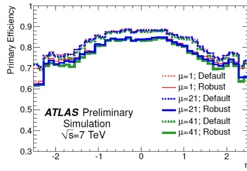
(b) Primary track reconstruction efficiency vs \eta
